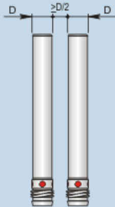
Side by side mounting
