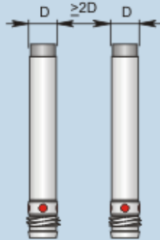
Side by side mounting
