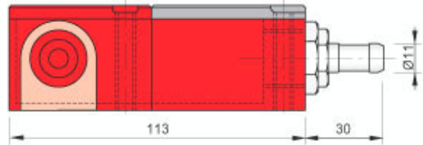
Version with cable exit - side view (IP 67)
